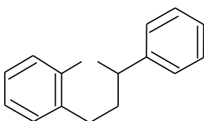
Flavan = 2 phenyl chroman
